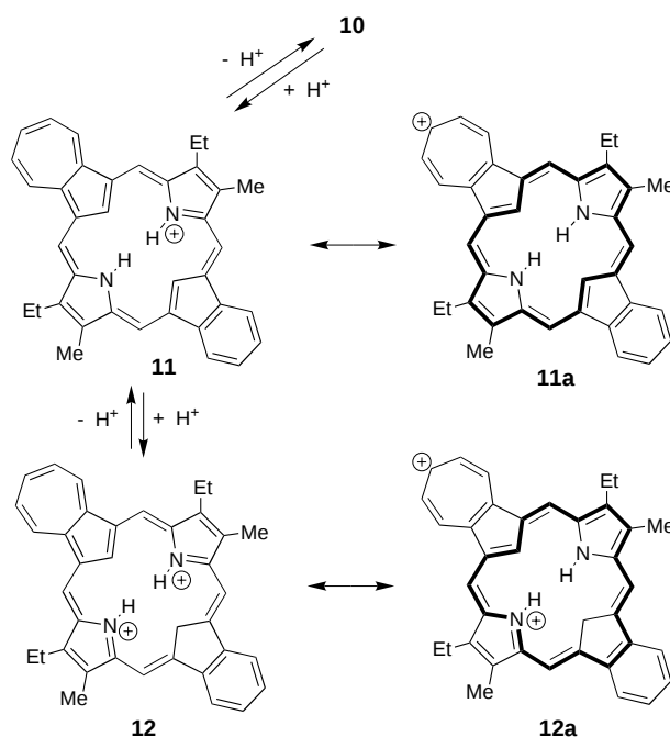
Scheme 3. Protonation of benzocarbazauporphyrin 11 .
